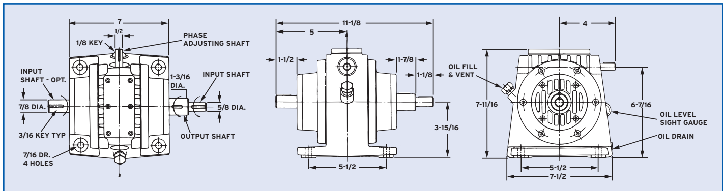
One Rotation of Adjustment Shaft, while running or stopped, provides approximately 3\frac{3}{4}^\circ Radial Movement of Output Shaft (96:1 Ratio)
