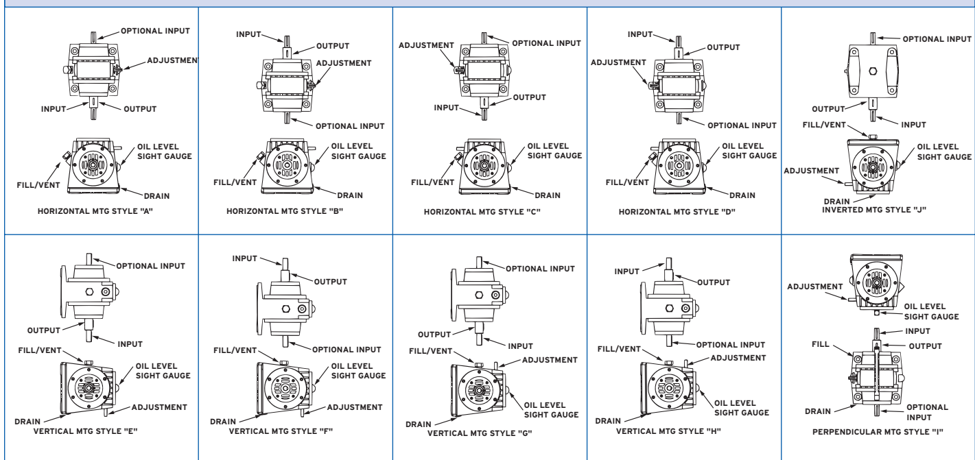
One Rotation of Adjustment Shaft, while running or stopped, provides approximately 3\frac{3}{4}^\circ Radial Movement of Output Shaft (96:1 Ratio)
