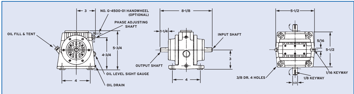
One Rotation of Adjustment Shaft, while running or stopped, provides approximately 4° Radial Movement of Output Shaft (88:1 Ratio)
